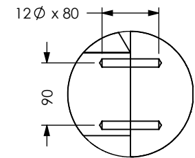
DETAIL C SCALE 2 : 15
