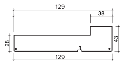
FRAME HEAD
