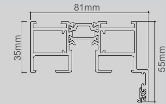
FRAME HEAD
